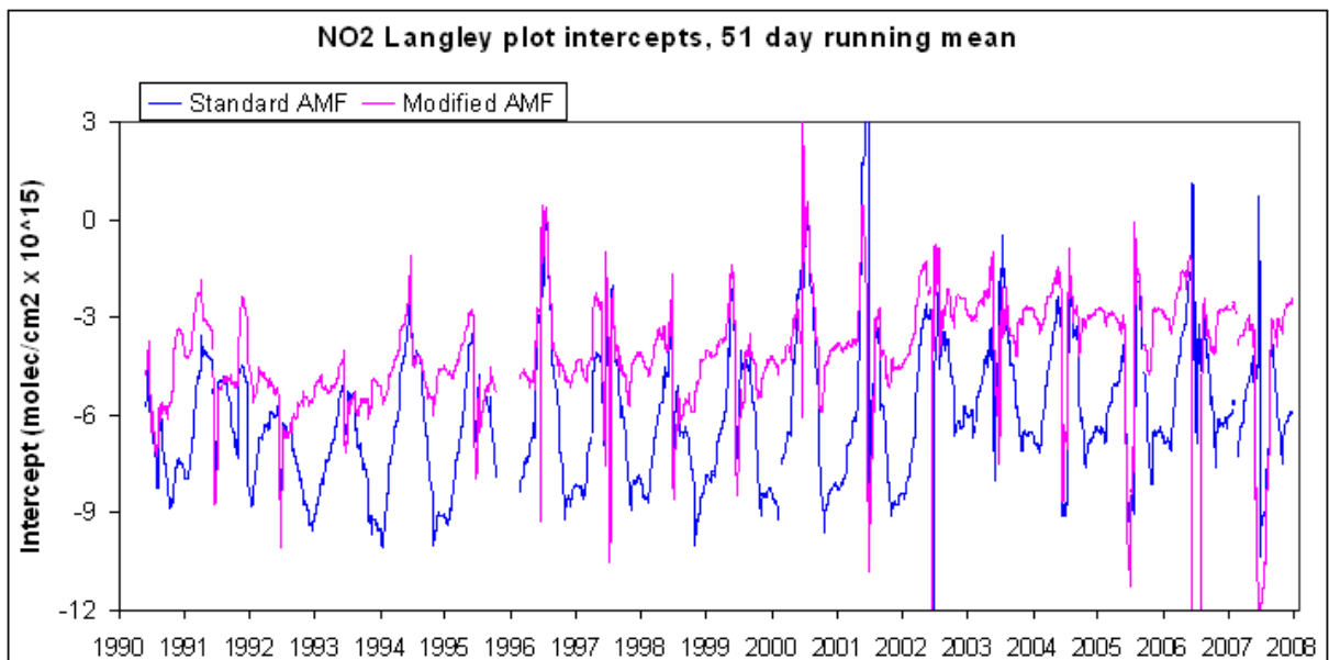
Fig. 3. The Langley plot intercepts produced by the analysis using unmodified and modified AMFs, with a 51 day running weighted mean. The modified AMFs produce much smaller intercepts, particularly at midsummer (note that the intercept equals the negative of the amount of \text{NO}_2 in the reference spectrum, plus any artefact). At midwinter the Langley plots are much poorer and give inaccurate intercept values because little of the \text{NO}_y is in the form of \text{NO}_2 , and the range of SZA, and hence AMF, is small.
