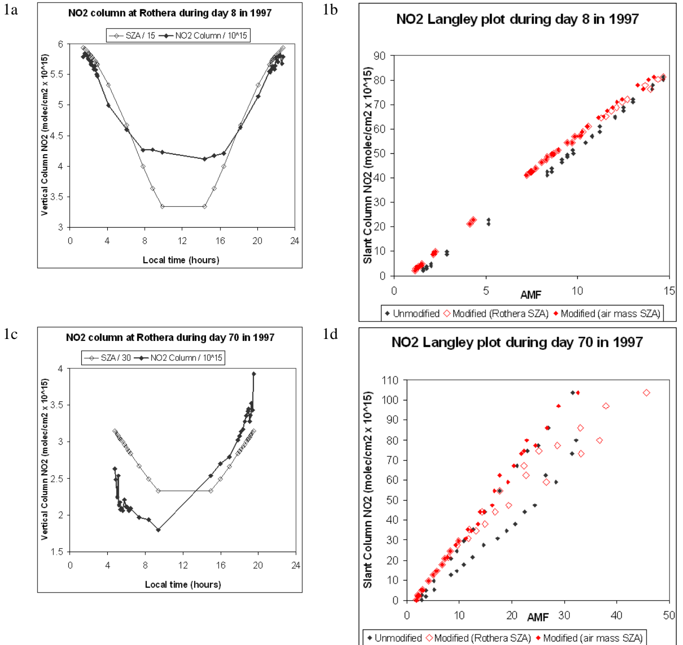
Fig. 1. Examples of the daily variation in NO 2 with time and SZA, and of the Langley plots produced for the analysis, for days 8 (a-b) and 70 (c-d) in 1997. Day 8 was in the summer when there was little N 2 O 5 , most of the variation was from the interchange between NO 2 and NO, and there is only a small difference between the morning and afternoon columns. However day 70 was in the autumn when most of the variation was from the interchange between N 2 O 5 and NO 2 , creating a large difference between the morning and afternoon columns. The Langley plots use unmodified Air Mass Factors (AMFs), AMFs modified by chemical ratios chosen from the Solar Zenith Angles (SZAs) at the spectrometer, and also AMFs modified by chemical ratios chosen from the mean SZAs for the air mass.
