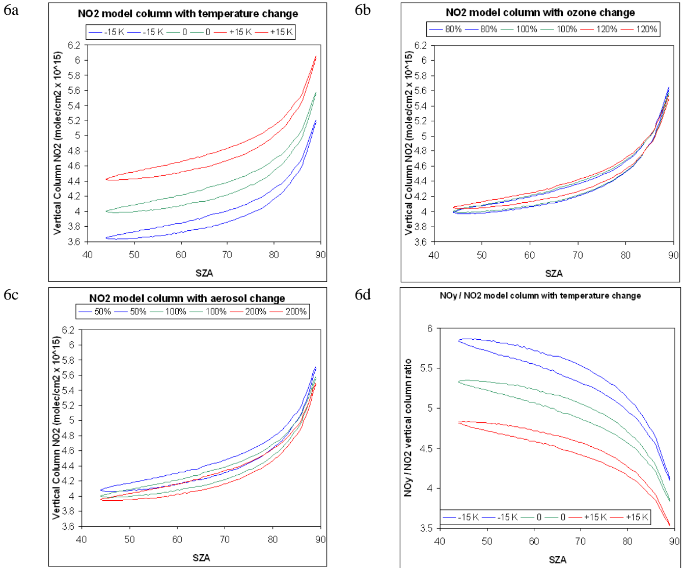
Fig. 6. The sensitivity of the box model \text{NO}_2 vertical column over Rothera in midsummer to temperature, ozone and aerosols, and the sensitivity of the \text{NO}_y / \text{NO}_2 ratio to temperature. Each shows the results from 3 simulations, with the unchanged climatology, and with the input values increased and reduced. (a) Stratospheric temperature increased and reduced by 15 K. (b) Ozone increased and reduced by 20% at all altitudes. (c) Aerosols doubled and halved at all altitudes (changes made to \text{H}_2\text{SO}_4 in the model). (d) The \text{NO}_y / \text{NO}_2 ratio in the 3 simulations at different stratospheric temperatures.
