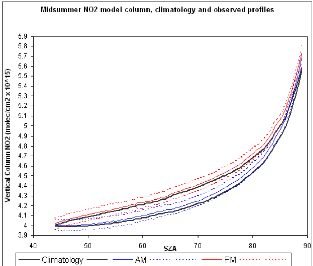
Fig. 7. The box model NO 2 vertical column over Rothera in midsummer, mean and standard deviation, using the observed temperature and ozone profiles (blue and red lines), and using the climatology (black line).
