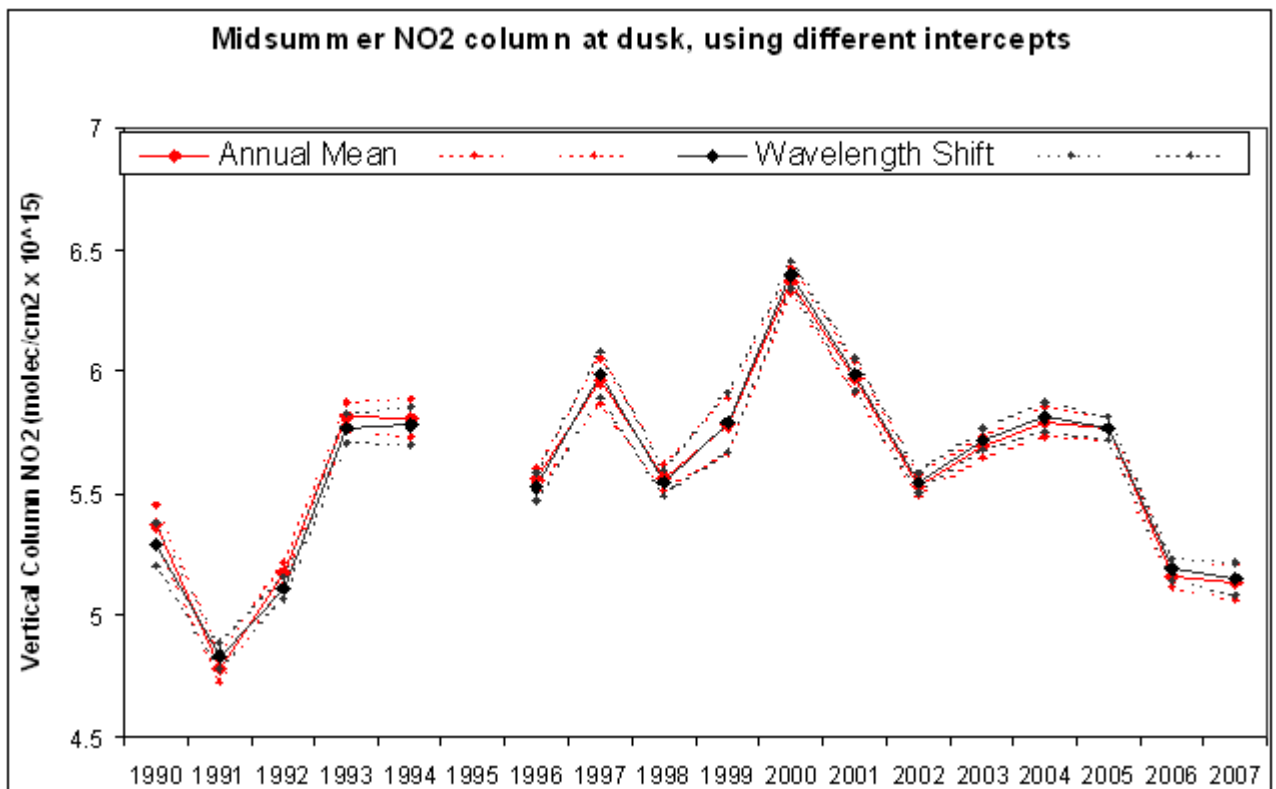
Fig. 5. The midsummer \text{NO}_2 vertical columns at twilight ( 87^\circ to 92^\circ SZA) for each year, weighted mean and standard deviation for the days 16 to 26 December. (a) Dawn and dusk columns calculated using annual weighted mean modified Langley plot intercepts, and (b) dusk columns calculated using annual mean intercepts, and daily intercepts estimated from the wavelength shift. There were no midsummer measurements in 1995.
