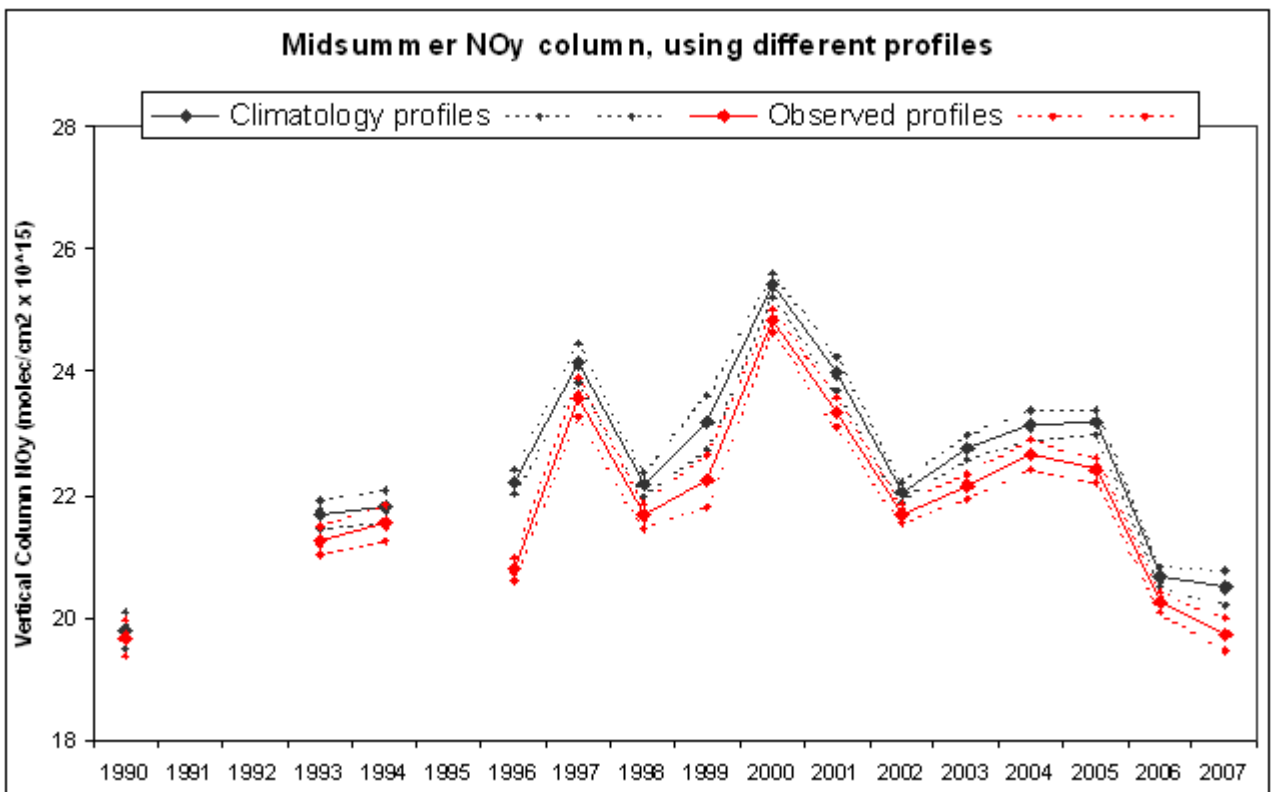
Fig. 9. The midsummer \text{NO}_y vertical columns, calculated from the \text{NO}_2 values at 89^\circ SZA in figure 8 and the box model \text{NO}_y / \text{NO}_2 ratio at 89^\circ for each year. (a) Interpolated dawn and dusk columns using the observed profiles, and (b) interpolated dusk columns using the observed and climatology profiles.
